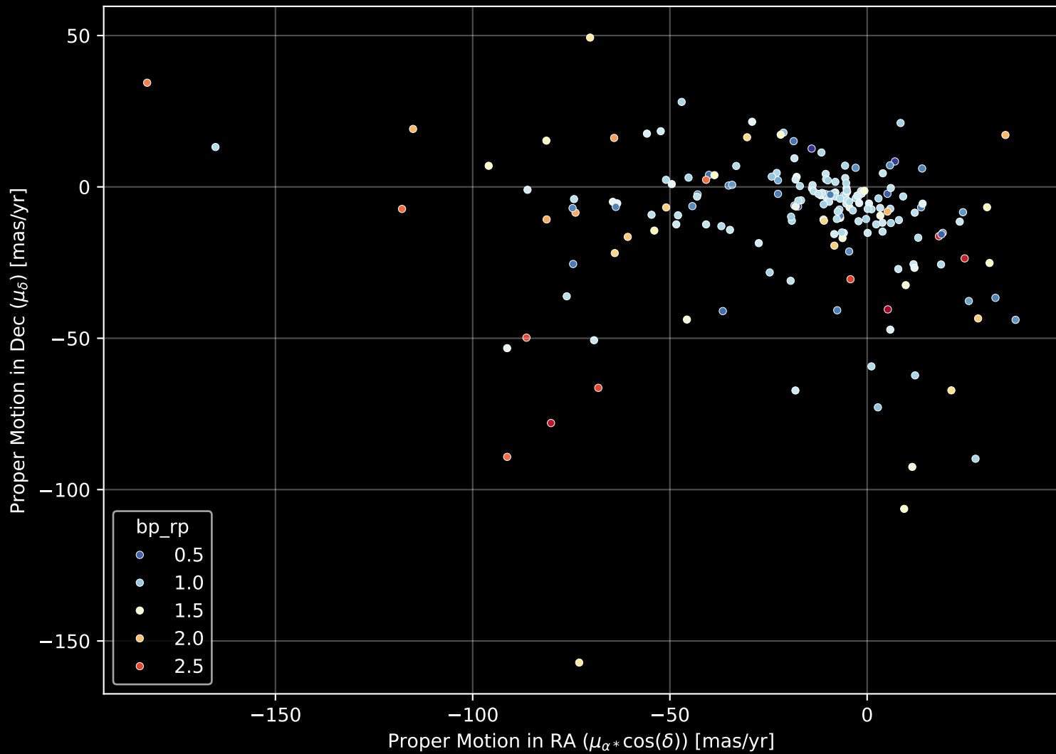
APOGEE DR17 Field: [280+60] Proper Motion Diagram (n= 190)
