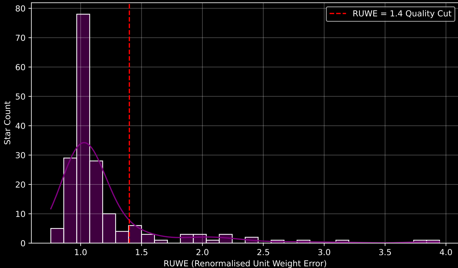
GAPOGEE DR17 Field [280+60] RUWE Distribution (n= 181)
