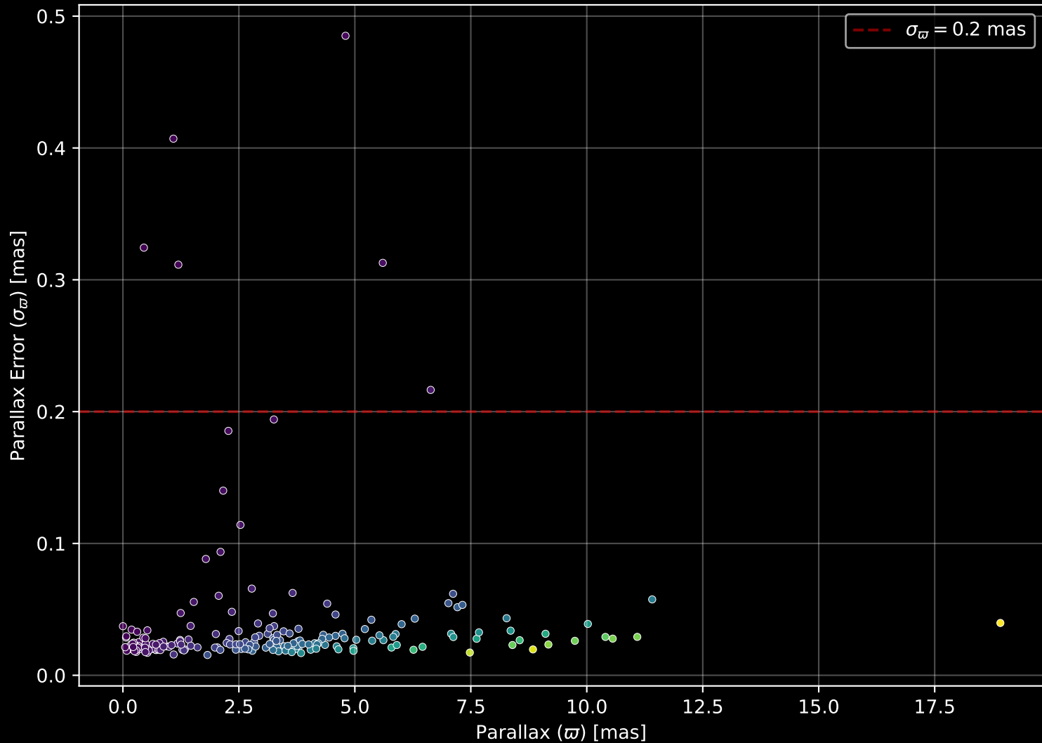
APOGEE DR17 Field: [280+60] Parallax Quality (n= 190)
