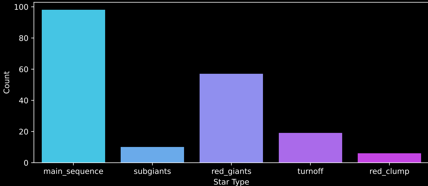
APOGEE DR17 Field: [280+60] Count plot of Star Type
