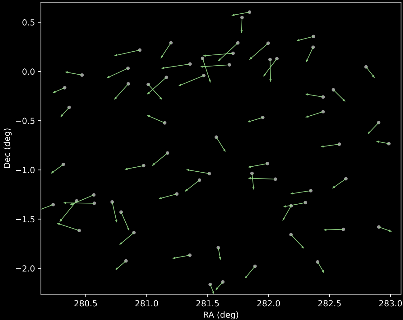
APOGEE DR17 Cluster 5 Proper Motion Vectors (n=63)
