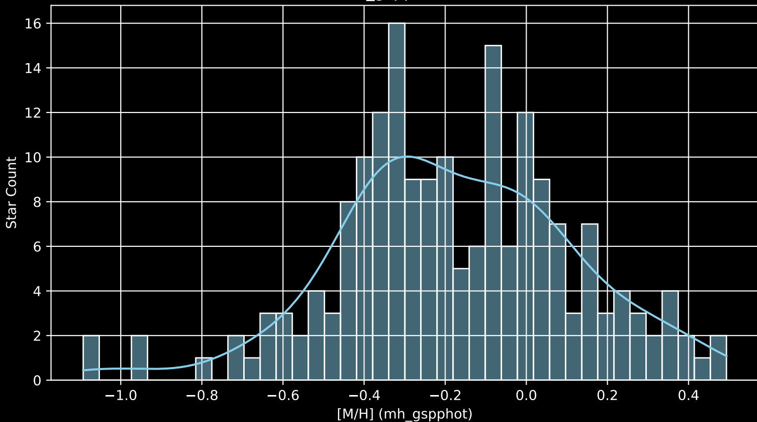
APOGEE DR17 Field: [280+60 [M/H] (mh_gspphot) (n= 188)
